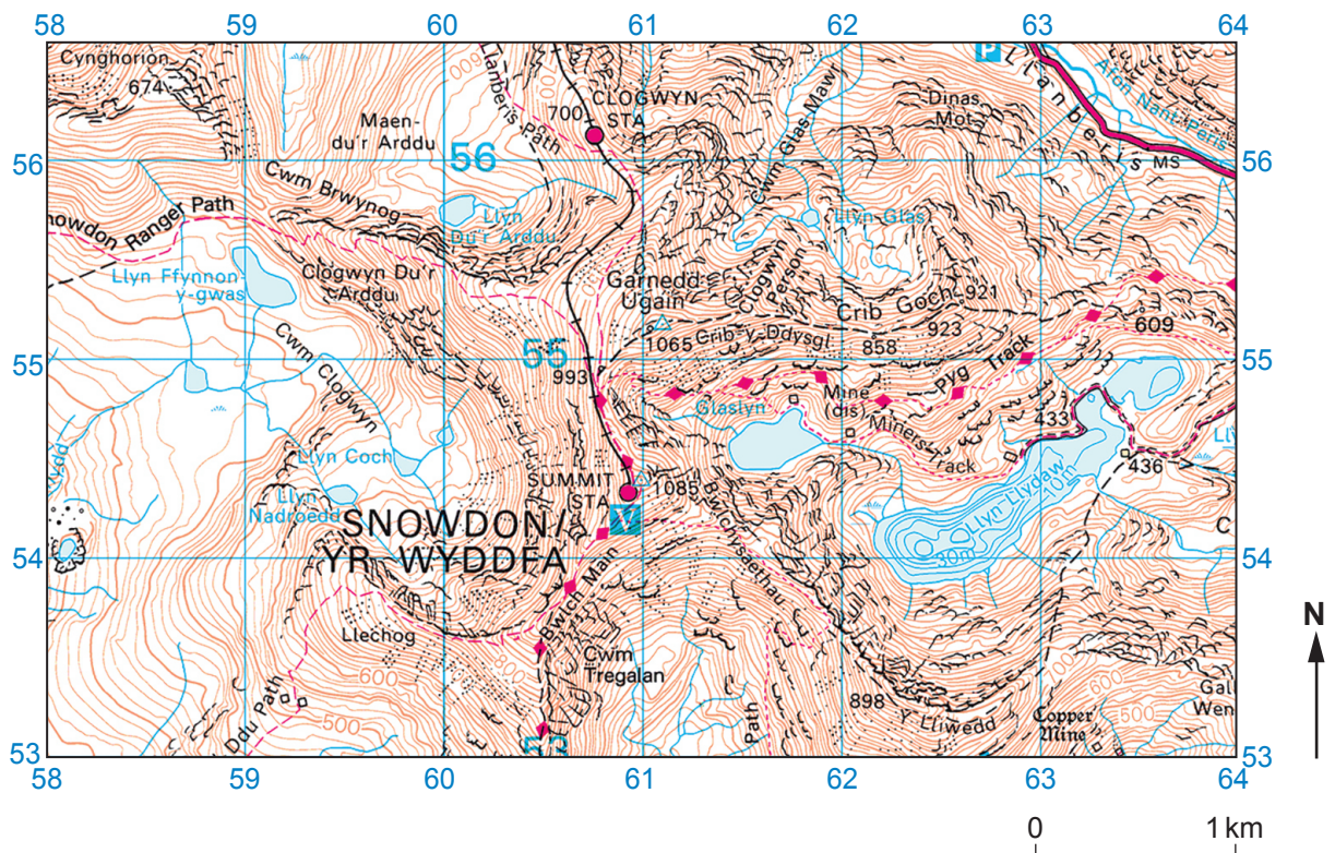
Figure 3: Part of the glaciated landscape of North Wales
